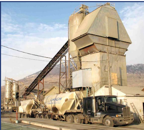
Figure 47. A redi-mix concrete and asphalt plant, and gravel pit along Yellowhead Highway 5 at Paul Lake Road. Sand and gravel deposits are sorted by screening into separate piles of gravel and sand, and used in the production of concrete.
