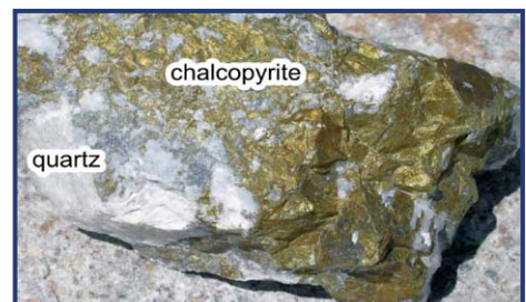
Figure 38. A rich sample of copper ore containing the brassy mineral chalcopyrite (copper-iron-sulphur) and white quartz. (Photo by R. Turner)
