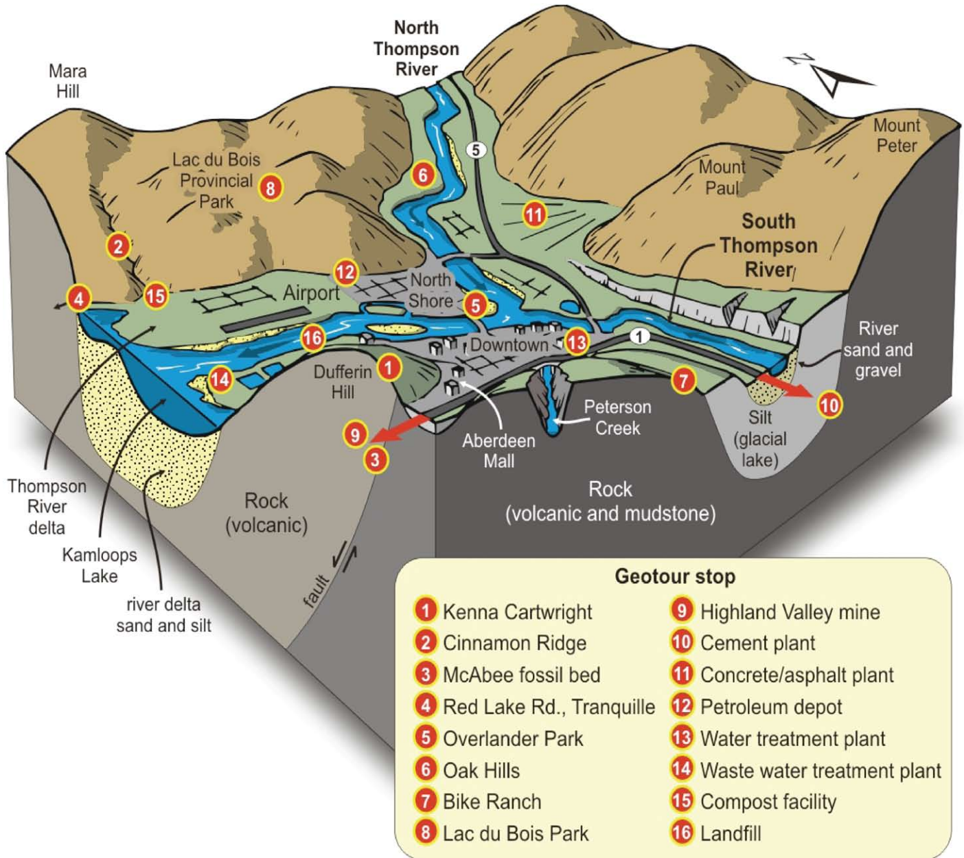
Figure 7. Stops in the Kamloops GeoTour guide are on a geological cut-away view of Kamloops. Three major types of geological materials underlie the Kamloops Region. Rock is the oldest material and it underlies the entire region and is dominantly volcanic rock and mudstones. Ice Age sediments form a widespread blanket over the plateau, and thick silt benches in the South Thompson River valley. Since the end of the last Ice Age, 10,000 years ago, the Thompson Rivers and their tributaries have eroded through the Ice Age sediments, and deposited modern sediments of sand, gravel, and silt in river plains, deltas, and lakes.
