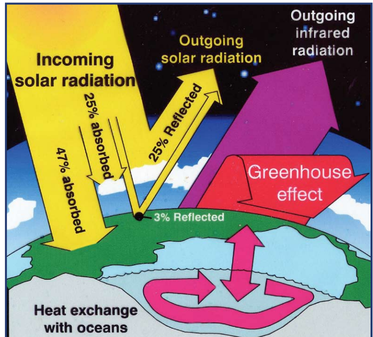
Figure 51. The production and burning of fossil fuels is rapidly adding carbon to the atmosphere. Fossil fuels represent carbon that once was part of the natural carbon cycle but long ago became stored in the Earth. Releasing this carbon into the Earth's atmosphere is upsetting the natural balance developed by nature, and allowing the levels of carbon to increase in the atmosphere. Carbon gases such as carbon dioxide and methane are referred to as "greenhouse" gases because of their natural ability to trap heat in the atmosphere. The build-up of these greenhouse gases in the atmosphere is causing surface warming of the planet Earth. Such global warming and climate change has a myriad of consequences, including melting of glaciers and ice caps, sea level rise, and changes in rainfall and storm patterns.
