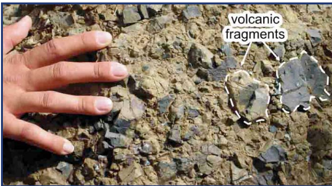
Figure 12c. Close up of fragmental volcanic rock exposed in canyon walls. The rock formed by explosive volcanic eruptions of rock fragments and ash 50 million years ago. (Photos by R. Turner)
