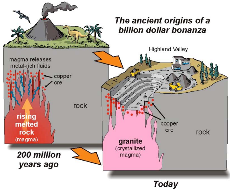
Figure 39. The origin of the Highland Valley mine.
