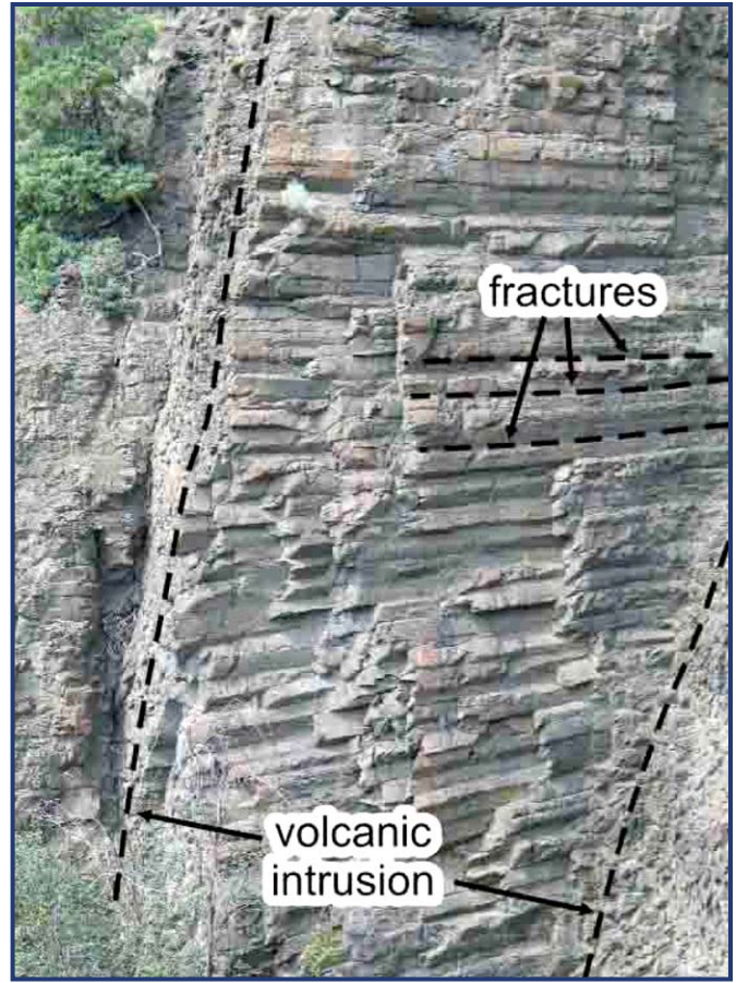
Figure 12b. Curious fractures that create column-like shapes in volcanic rock formed by the cooling and contraction of the molten lava. The molten lava intruded along a steep fracture in the ancient volcano, then cooled to form volcanic rock.
