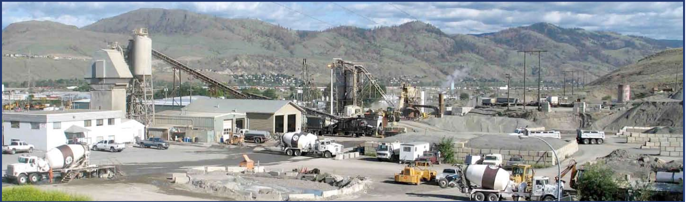
Figure 47. A redi-mix concrete and asphalt plant, and gravel pit along Yellowhead Highway 5 at Paul Lake Road. Sand and gravel deposits are sorted by screening into separate piles of gravel and sand, and used in the production of concrete.
