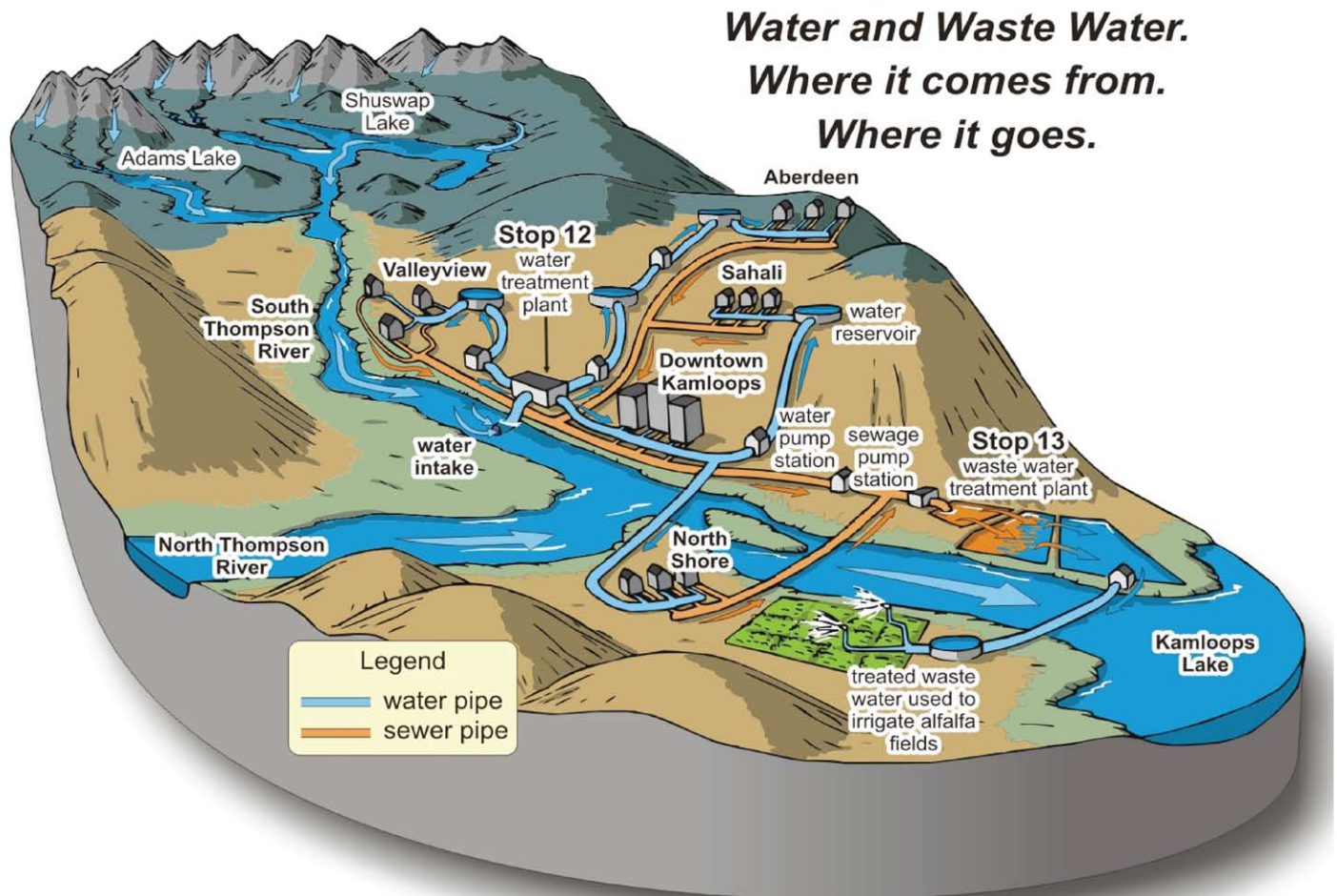
Figure 53. Kamloops water supply is drawn from the South Thompson River through an intake pipe just upstream of the downtown area. The river is fed by snowmelt and rainfall within its watershed. The water is filtered and pumped by pipe (blue) throughout the city, including areas as much as 500 metres above the river. Waste water from homes and businesses is collected in a network of sewer pipes (orange) that carry waste water to a treatment plant west of the city. Treated water is either returned to the river or used to irrigate hay crops.
