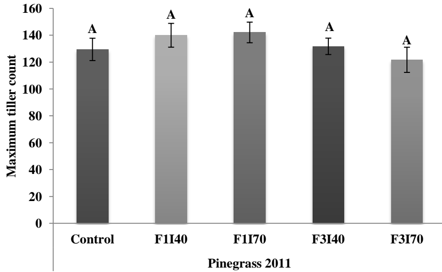
Appendix 4: Maximum tiller counts for pinegrass in 2011. Letters denote significance ( P < 0.05 ). Data in graph represents untransformed data and error bars are for untransformed data while statistical analysis was done with transformed data. Control – No clipping, F1I40 – clipped once at 40% removal, F1I70 – clipped once at 70% removal, F3I40 – clipped three times at 40% removal, F3I70 – clipped three times at 70% removal.
