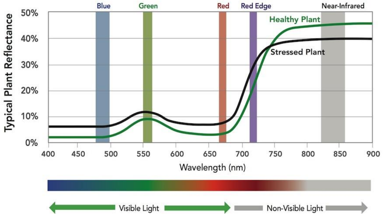
Figure 1.2: An example of a typical plant reflectance curve detailing the wavelengths and position of visible and non-visible light (Micasense Inc.) (Parker 2019).
