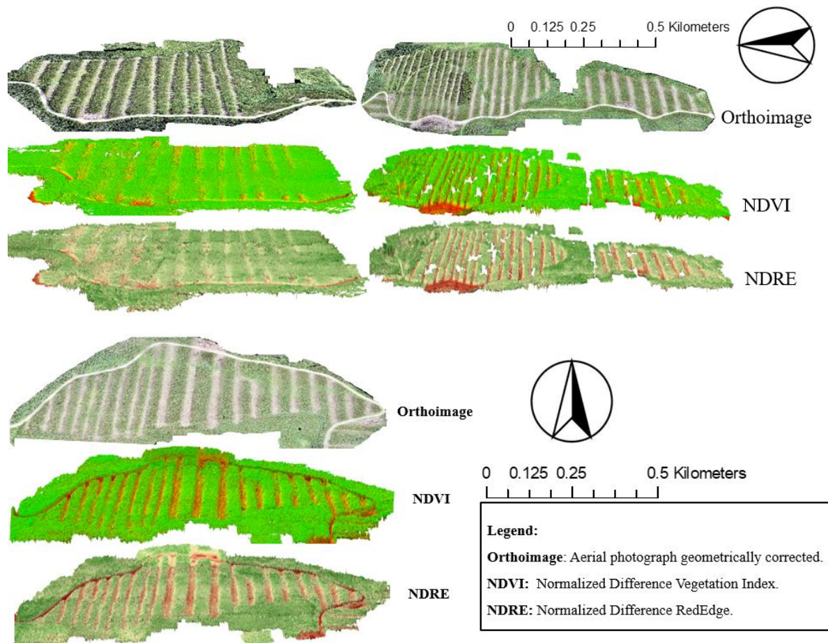
Figure 2.18 Orthomosaic images with corresponding NDVI and NDRE indexes of the three adjacent forest sites located in Goudie, East Kelowna, British Columbia. Orthoimages and multispectral sensor images were taken post timber harvest.
