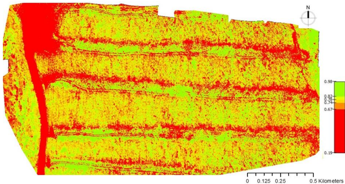
A.13. An NDVI map example that shows soil compaction in the strips post timber harvesting.
