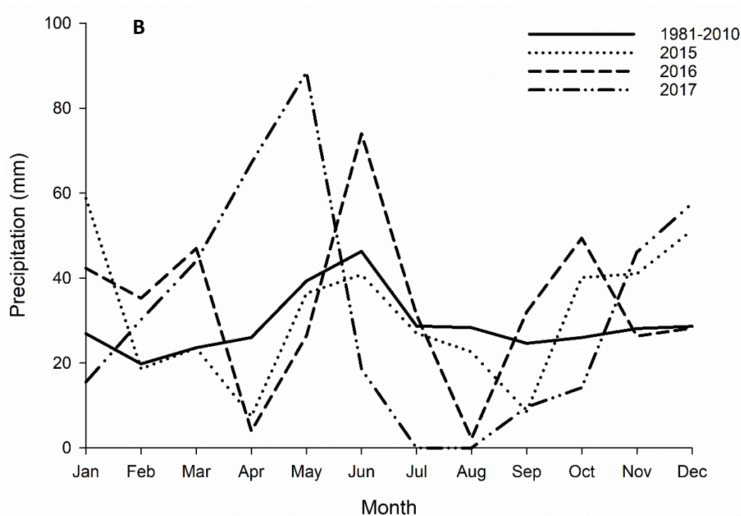
Figure 1.5. A) Mean monthly temperature ( ^{\circ}\text{C} ) and B) total monthly precipitation (mm) in the South Okanagan during the study years (2015, 2016, and 2017) compared to the 30-year mean (1981-2010) as measure at the Penticton Regional Airport, British Columbia, Canada ( 49^{\circ}\text{N} , 119^{\circ}\text{W} ; Environment and Climate Change Canada 2018).
