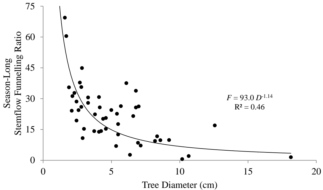
Figure 3.4. Season-long stemflow funnelling ratios versus tree diameter for all healthy lodgepole pine trees in Plots E, D, C, and B.
