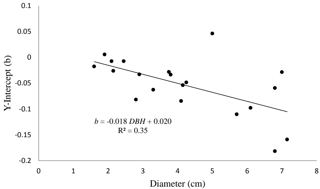
Figure 3.6. Intercept values versus diameter showing a weak linear relationship and not the power relationship shown by Park and Hattori (2002).
