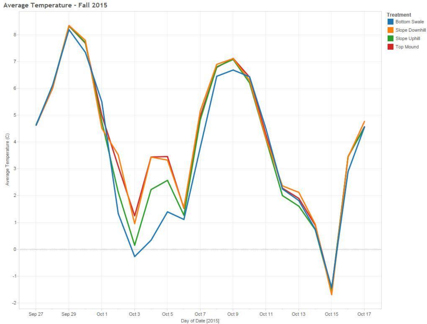
Figure 4: Average daily near surface air temperature (°C), September 27-October 17 2015 (n=8). Letters indicate significant differences between means (Tukey HSD) at \alpha=0.05 .
