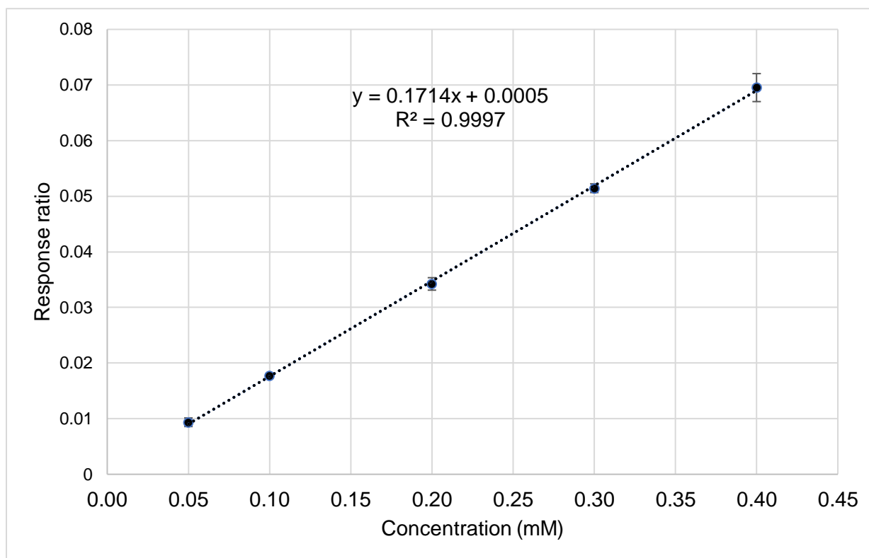
Figure S2. Octanol standard curve of 50 to 400 \mu\text{M} calculated from the response ratio of octanol to decanal. Standards were prepared by diluting octanol working stocks to concentrations of 50, 100, 200, 300 and 400 \mu\text{M} in ethyl acetate. Error bars represent standard deviation ( n=3 ).
