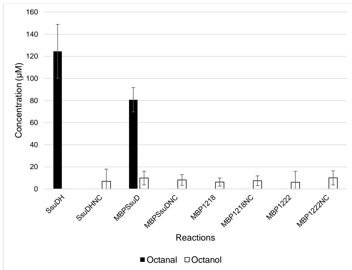
Figure 17. Concentration of octanal and octanol in reactions challenged with octane sulfonate. Enzyme names represent the catalyst used in the reaction and NC denotes no catalyst added. Ethyl acetate blanks were regularly run every six samples to identify contamination between samples. No hexanal, octanal, octanol or decanal was observed in blanks. Error bars represent standard deviation (n=3).
