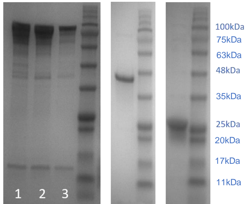
Figure 14. Partial purification of MBP1835 (1), MBP1666 (2) and MBP205 (3), purification of SsuDH (middle) and FreH (Right). The protein ladder is the BLUelf Prestained Protein ladder (FroggaBio, Toronto, ON). MBP1835 is predicted to be 95.11 kDa; MBP1666, 93.82 kDa; MBP205, 95.12 kDa; SsuDH, 43.45 kDa; and FreH, 29.96 kDa.
