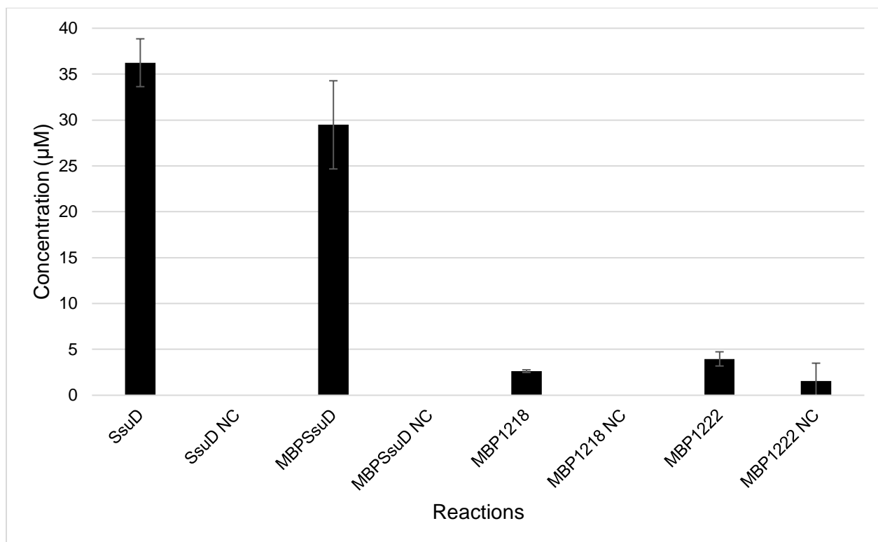
Figure 20. Concentration of sulfite in ethyl acetate extracted reactions challenged with 6:2 FTSA. Reactions were incubated with DTNB for 5 minutes at room temperature prior to measurement. Enzyme names represent the catalyst used in the reaction and NC denotes no catalyst added. Error bars represent standard deviations (n=3). MBP1222 and MBP1222NC are not statistically different.
