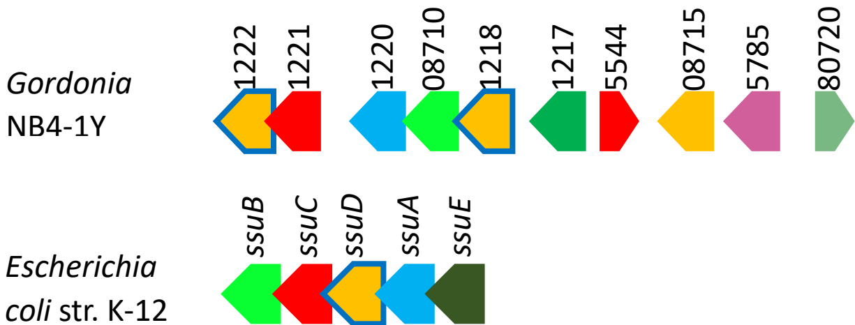
Figure 6. Genomic context surrounding the genes encoding ISGA 1218 and 1222 (top) in Gordonia NB4-1Y and ssuD (bottom) in E. coli K-12. The numbers above each gene represent their respective ISGA number. In the region surrounding the genes encoding ISGA 1218 and 1222 there is predicted to be three ABC type transporter proteins ( 1221 , 1220 and 08710 ), a tyrosine phosphatase ( 1217 ), a tetR family transcriptional regulator ( 5544 ), a dsbA oxidoreductase ( 08715 ), a lysR family transcriptional regulator ( 5785 ) and a FAD linked oxidase ( 80720 ). The region surrounding ssuD in E. coli encodes three aliphatic sulfonate transporter proteins ( ssuB , C , A ) and an FMN reductase ( ssuE ). Blue trimmed genes are reference monooxygenases.
