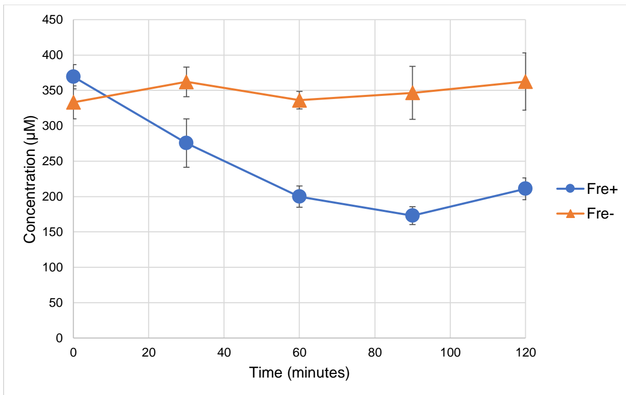
Figure 21. Concentration of sulfite in reactions with and without FreH. Fre+ indicates the presence and Fre- indicates the absence of FreH. Assays were carried out in triplicate and error bars represent standard deviations (n=3).
