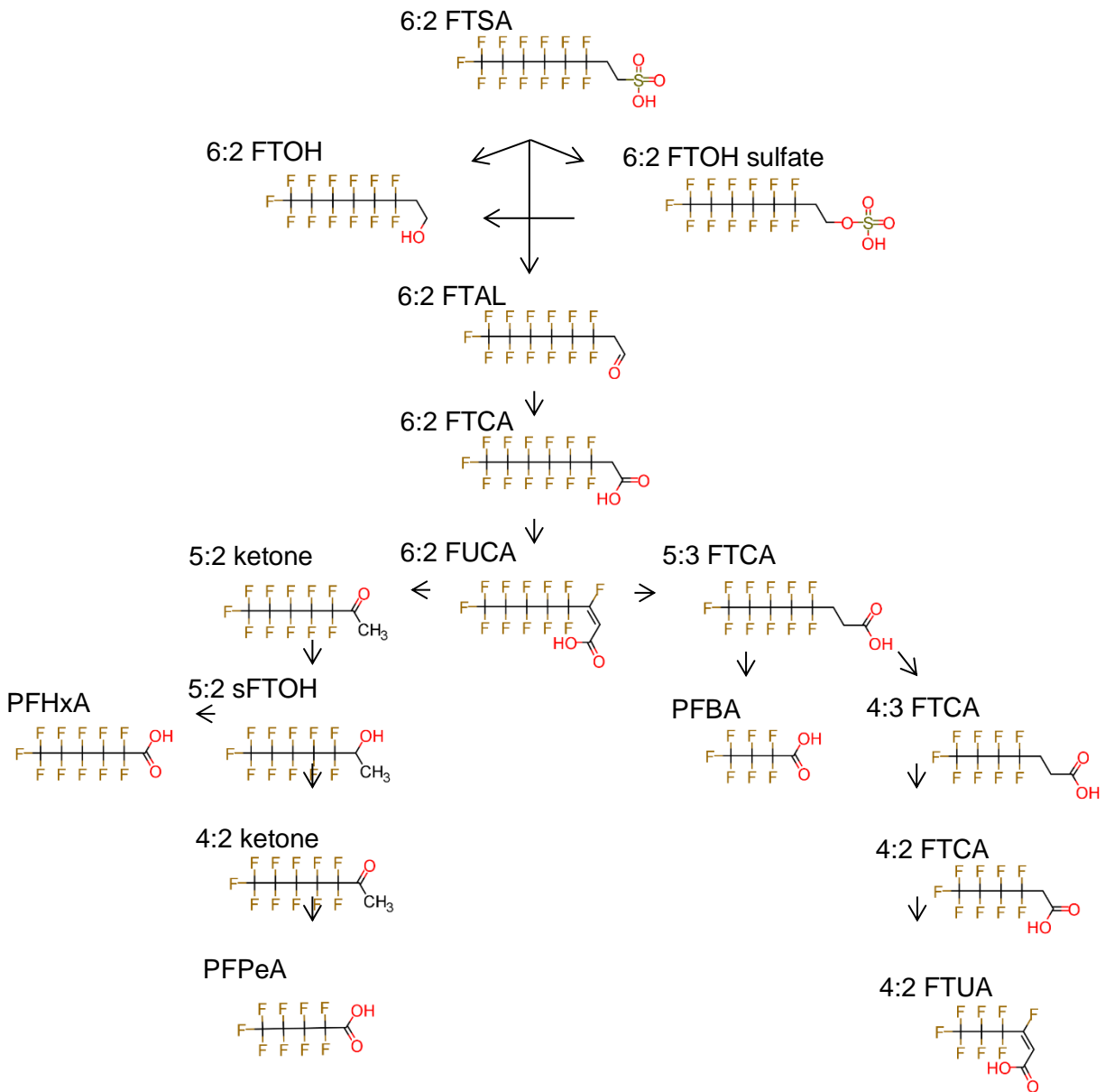
Figure 5. Degradation pathway of 6:2 FTSA by Gordonia NB4-1Y under sulfur limiting conditions; pathway adapted from Shaw et al. (2019). Acronyms not described in Figure 4 are FTOH sulfate (fluorotelomer sulfate ester).
