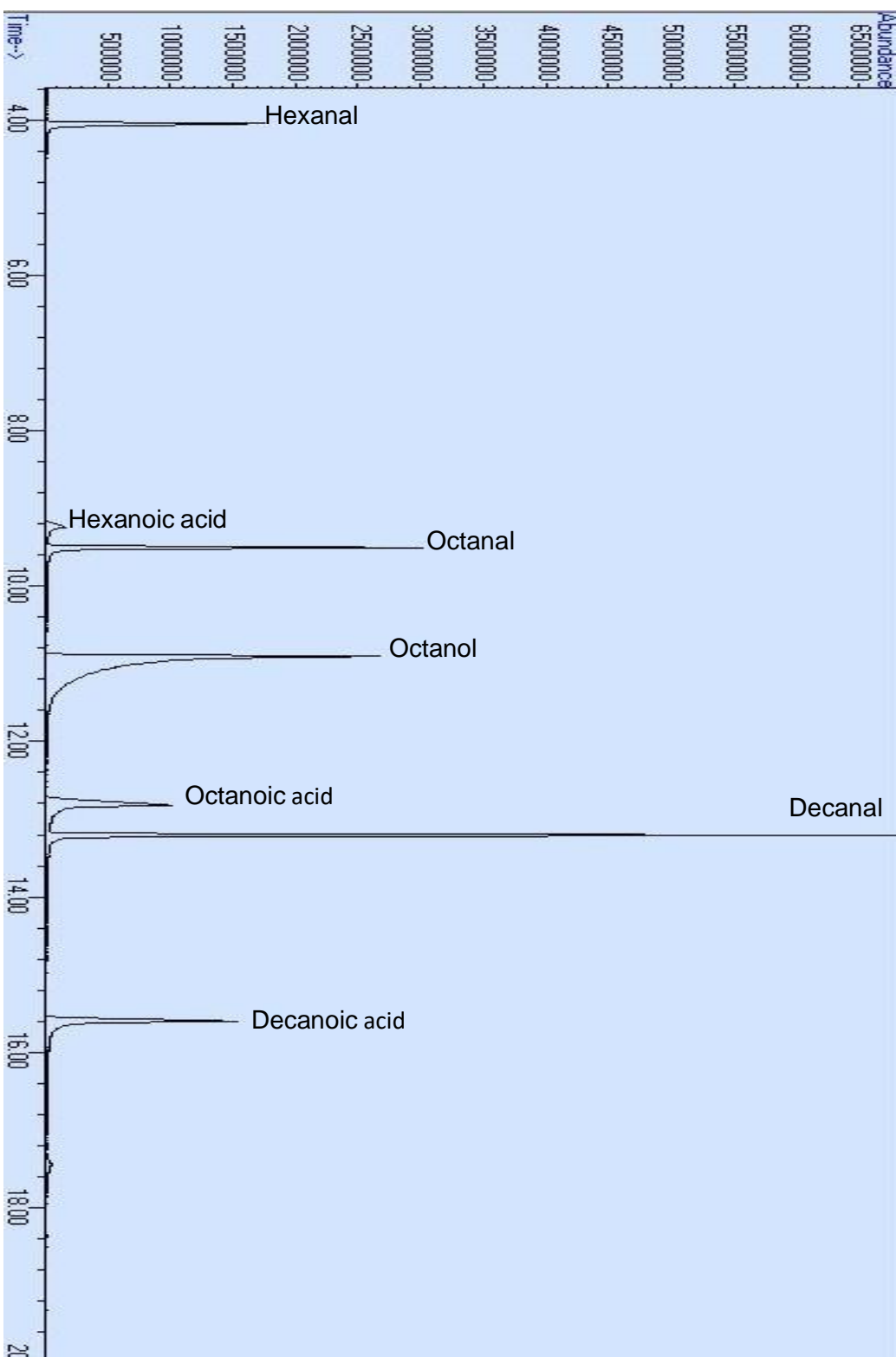
Figure S4. GC-MS chromatogram of all organic analytical standards used in this study. Percent probability of each peak when search against the National Institute of Standards and Technology (NIST) mass spectra library are as follows: hexanal – 89.1%, hexanoic acid – 85.8%, octanal – 88.5%, octanoic acid – 95.1%, octanol – 49.5%, decanal – 83.4% and decanoic acid – 92.2%.
