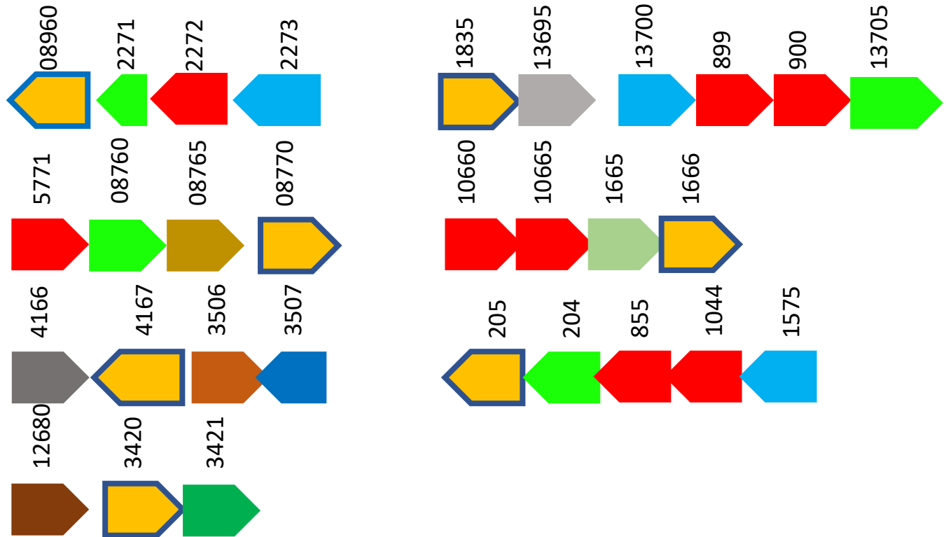
Figure 7. Genomic context of ssuD -like monooxygenases (left) and annotated alkanesulfonate monooxygenase (right) in the genome of Gordonia NB4-1Y. The numbers above each gene correspond to their respective ISGA number and are annotated as follows: 08960 : LLM class flavin-dependent oxidoreductase; 2271 : ABC transporter ATP-binding protein; 2272 : ABC transporter permease; 2273 : aliphatic sulfonate ABC transporter substrate-binding protein; 5771 : iron ABC transporter permease; 08760 : ABC transporter ATP-binding protein; 08765 : hypothetical protein; 08770 : LLM class flavin-dependent oxidoreductase; 4166 : endonuclease/exonuclease/phosphatase family protein; 4167 : LLM class flavin-dependent oxidoreductase; 3506 : acetyltransferase; 3507 : 4-hydroxybenzoate 3- monooxygenase; 12680 : ketopantoate reductase family protein; 3420 : LLM class flavin-dependent oxidoreductase; 3421 : DUF1684 domain-containing protein; 1835 : alkanesulfonate monooxygenase; 13695 : oxidoreductase; 13700 : ABC transporter substrate-binding protein; 899 : ABC transporter permease; 900 : ABC transporter permease; 13705 : ABC transporter ATP-binding protein; 10660 : ABC transporter permease; 10665 : ABC transporter permease; 1665 : acyl-CoA dehydrogenase; 1666 : alkanesulfonate monooxygenase; 205 : alkane sulfonate monooxygenase; 204 : ABC transporter ATP-binding protein; 855 : ABC transporter permease; 1044 : ABC transporter permease; 1575 : peptide ABC transporter substrate-binding protein.
