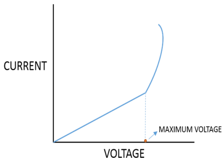
Figure 2.4. Ohm's law plot (Baker, 1995).
