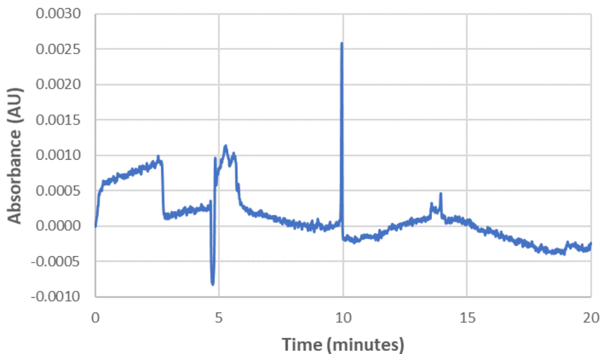
Figure 4.6. CE electropherogram of mussel sample #116 (3 MP count) collected from Duncan, BC, acidified for microplastic particle analysis and provided for BPA analysis. The pH of the sample was adjusted with NaOH and tested to be basic. The area of the peak at approximately 10 min was found to be 6957.
