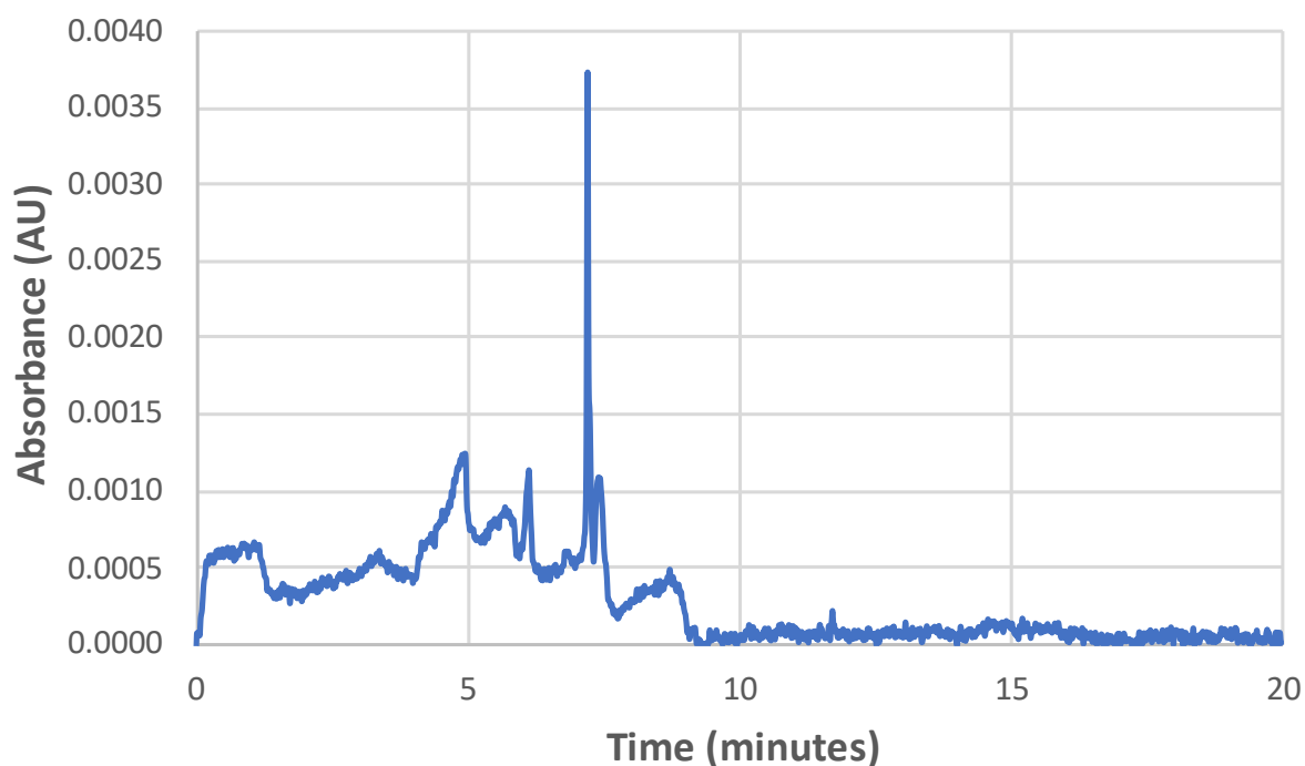
Figure 4.4. Electropherogram of mussel sample #109 collected from Oak Bay, BC. The sample was digested in nitric acid for microplastic particle analysis (2 MP count) and analysed by CE without pH adjustment. The large peak at 7.3 min was labeled by the CE analysis software with an area of 7472.
