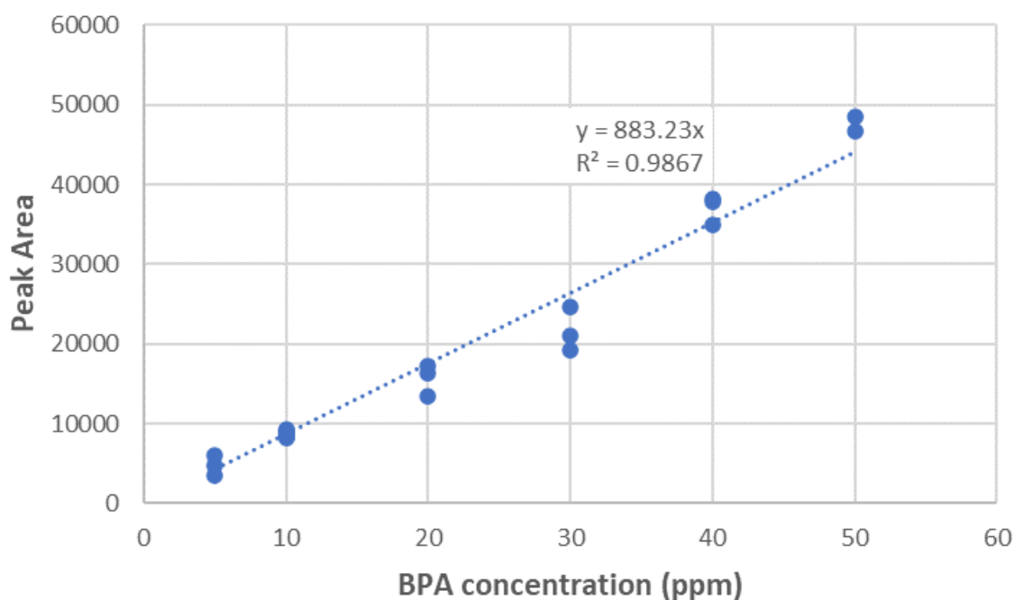
Figure 4.1. The calibration curve for BPA concentrations from 5 ppm to 50 ppm developed with the method used in this study.
