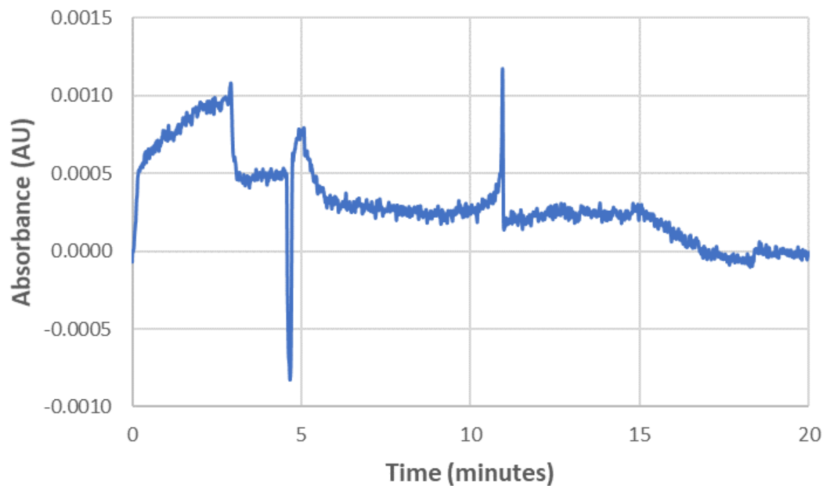
Figure 4.5. CE electropherogram of mussel sample #116 (3 MP count) collected from Duncan, BC, acidified for microplastic particle analysis and provided for BPA analysis. The pH of the sample was less than one and left unadjusted for CE analysis. The area of the peak at approximately 11 min has an area of 2617.
