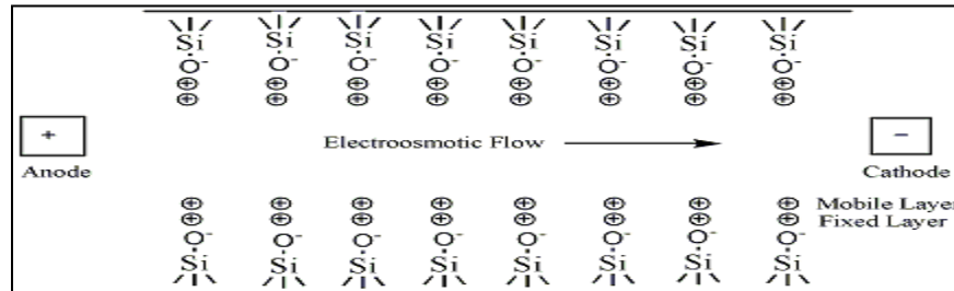
Figure 2.1. Double layer formed within capillary (Baker, 1995)
