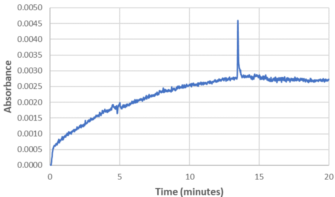
Figure 4.2. The electropherogram of the 10 ppm BPA standard as a sample of the data used to generate the calibration curve shown in Figure 7.
