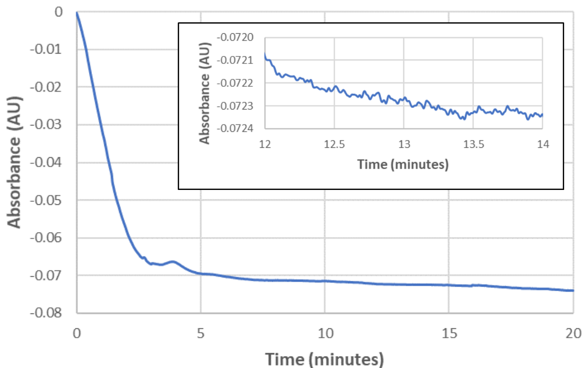
Figure 4.3. Sample electropherogram for CE analysis of Kamloops municipal tap water taken from the staff lunchroom in the Old Main building on the Thompson Rivers University campus showing no BPA detected. The peak for BPA is expected at about 13 min. The insert shows an expanded view from 12 min to 14 min.
