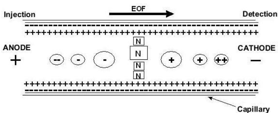
Figure 2.2. A diagram depicting EOF including the separation of ions based on size and charge between the anode and cathode (Laboratoire Suisse d'Analyse du Dopage, 2008) .
