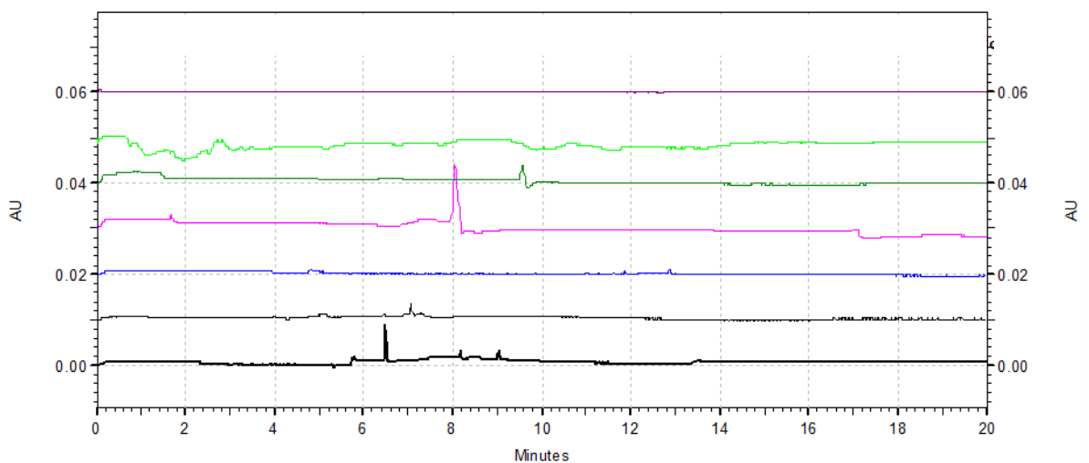
Figure B.4. Mussel sample electropherograms for samples: #109 pH unadjusted (black); #116 pH unadjusted (grey); #116 pH adjusted >6 (blue); #52 pH 6 (pink); #46 pH 3 (dark green); #46 pH 6 (bright green) and #46 pH unadjusted (purple). The pH of samples unadjusted were analysed as provided, pH <1.
