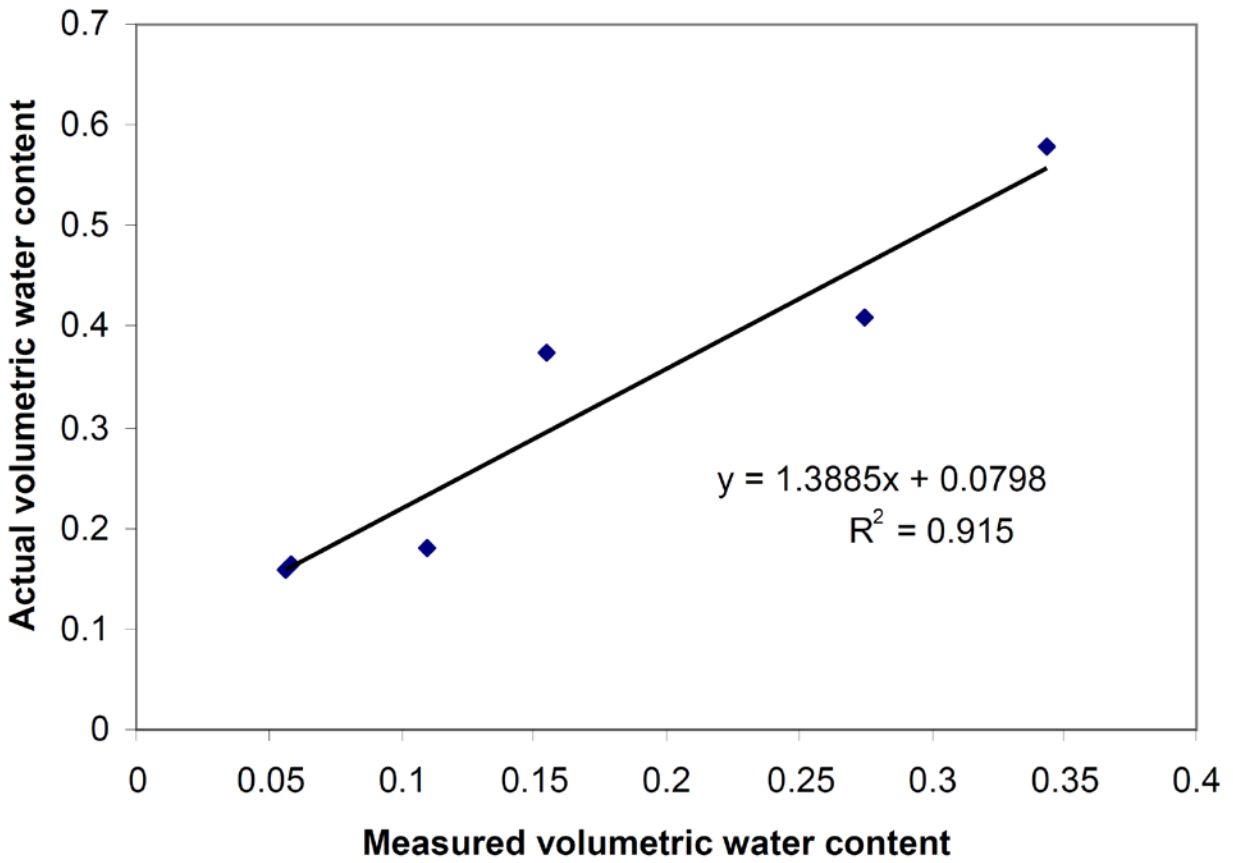
Figure A1.1 Plot from excel of actual volumetric water content plotted against the measured volumetric water content. The equation in the figure is the formula required to adjust field readings.
