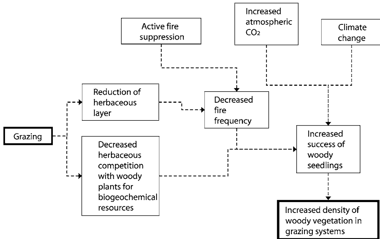
Figure 5.6.1-5-1: Processes contributing to woody encroachment in semi-arid systems. Climate change is expected to lead to an increased success of woody seedlings, such as sagebrush (From Asner et al. 2004).
