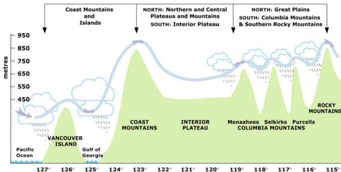
Figure 1.1: Longitudinal cross section of southern British Columbia (Williams 1982).
