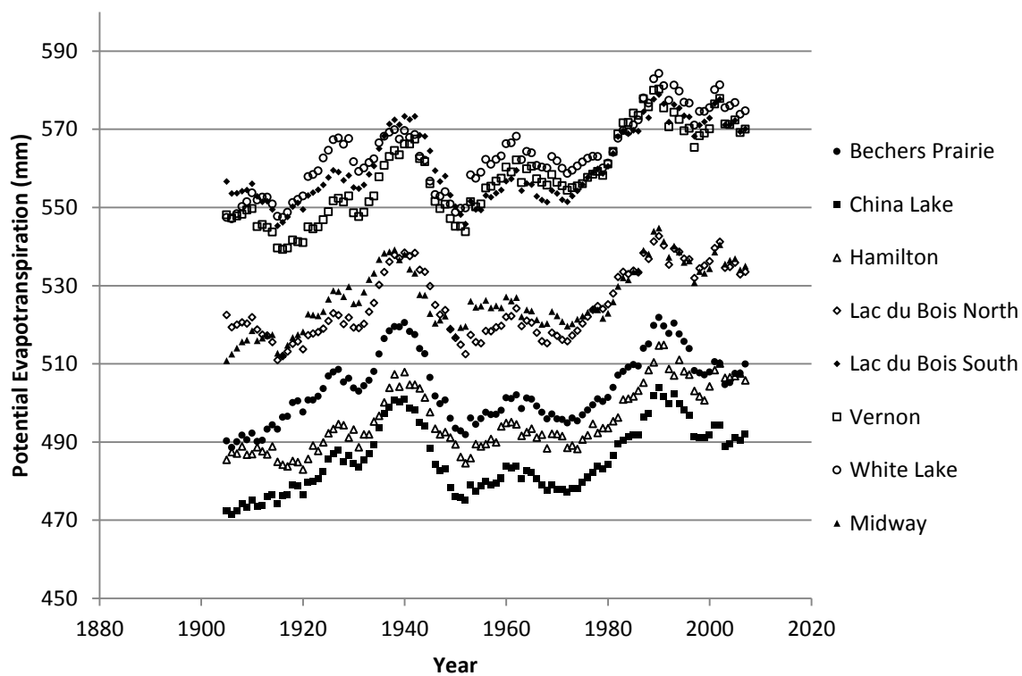
Figure 2.4: Ten year running means of potential evapotranspiration (PET) for long term ClimateWNA data from eight semi-arid grassland sites in BC. The linear trend since 1905 is positive and significant ( p < 0.001 ) for all sites.
