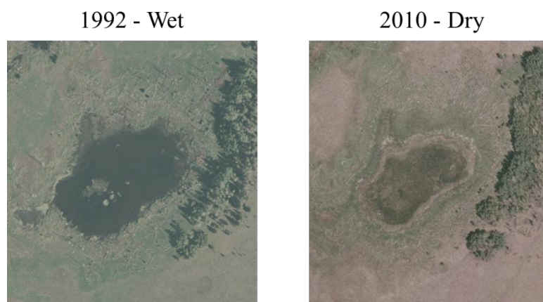
Figure 2.2: Example of a pond from the Becher's Prairie site that was wet in 1992 and dry in 2010. The total number of ponds containing water in each site in the 1990s were compared to the 2010 images to determine change in status (wet/dry).
