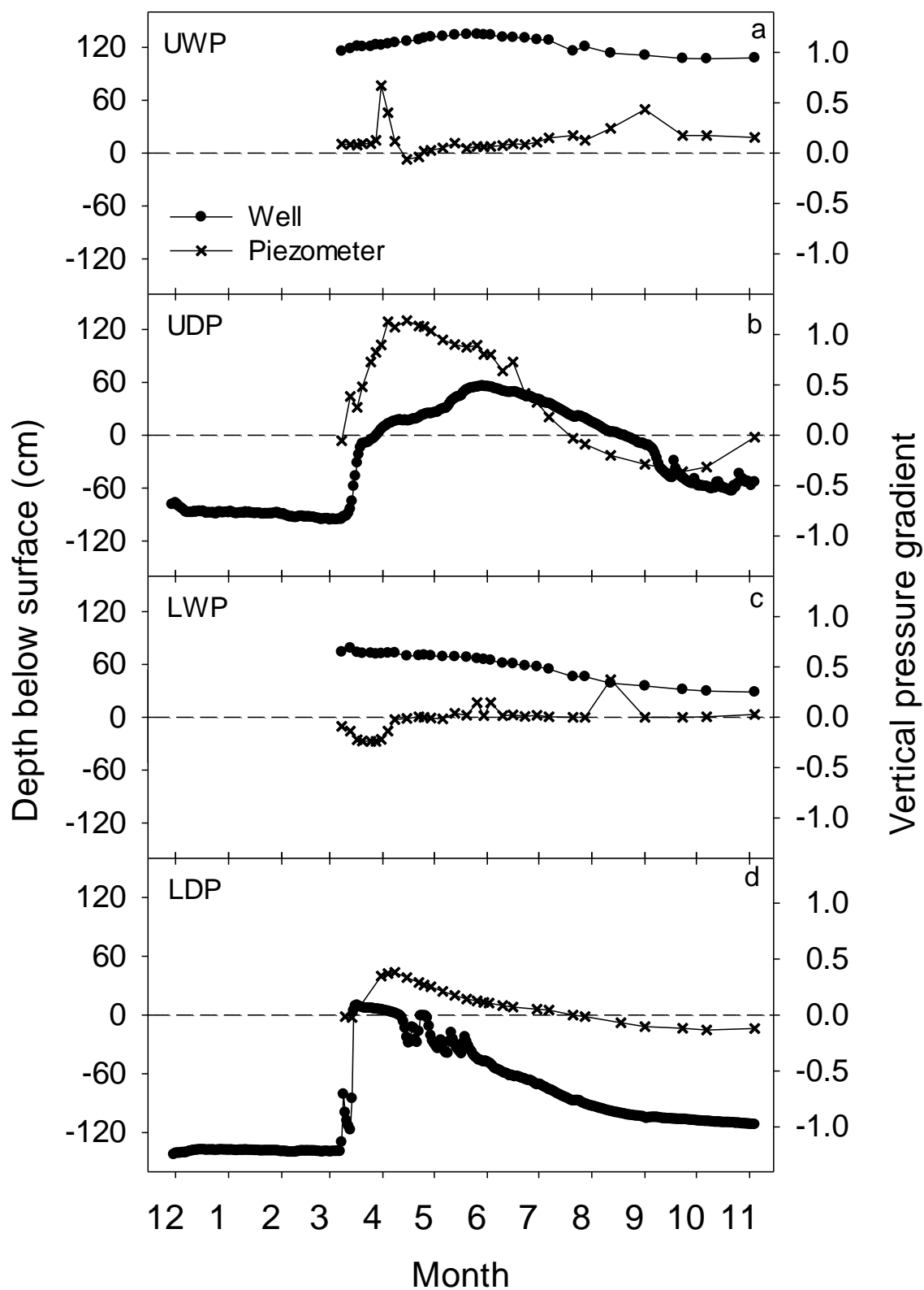
Figure 3.3: Depth of the water table at the middle wells (M) relative to the ground and the vertical pressure head gradient measure at M for all ponds.
