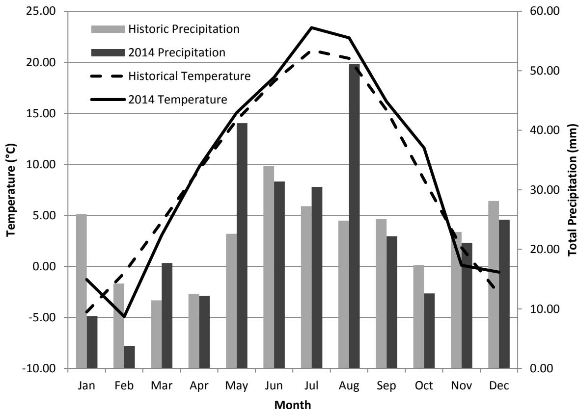
Figure 3.2: 2014 and historic (1951 - 2012) average monthly temperature and total monthly precipitation from the Kamloops Airport weather station.
