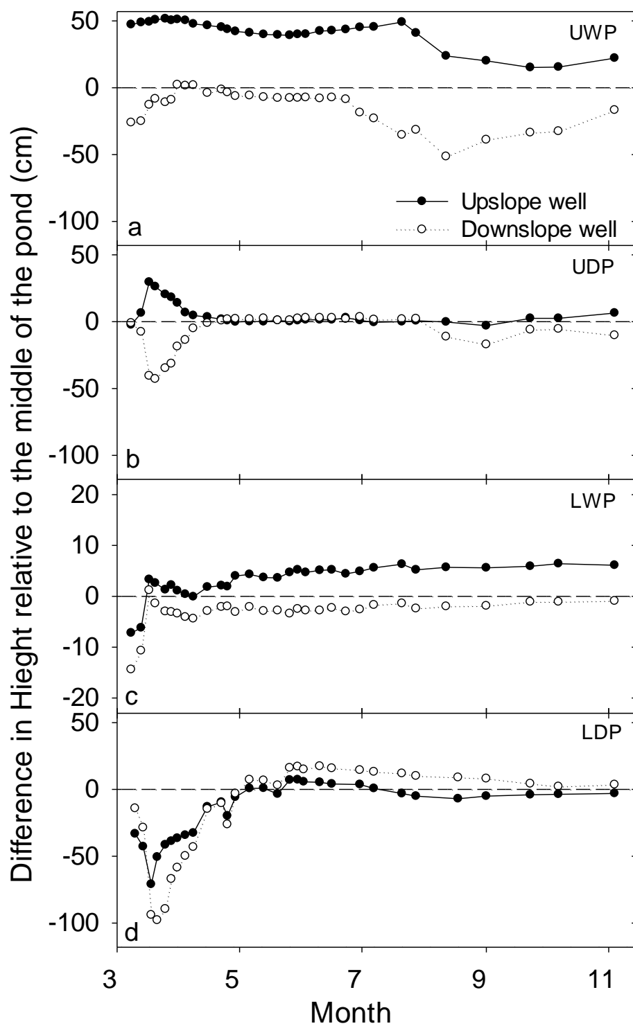
Figure 3.4: Depth of the water table of the upslope well (N) and the downslope well (S) relative to the middle well (M). Note: (c) has a different scale on the y-axis to better visualize the data.
