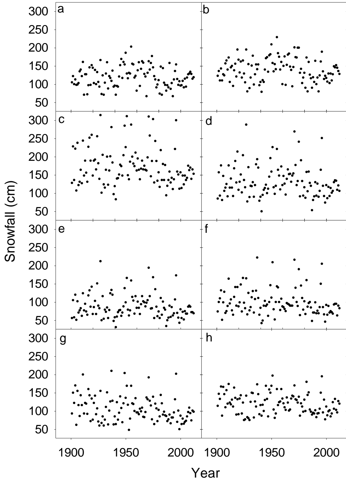
Figure 2.5: Total annual snowfall at eight semi-arid grassland sites in BC; (a) Becher's Prairie, (b) China Lake, (c) Hamilton Commonage, (d) Lac du Bois North, (e) Lac du Bois South, (f) Vernon Commonage, (g) White Lake, (h) Midway.
